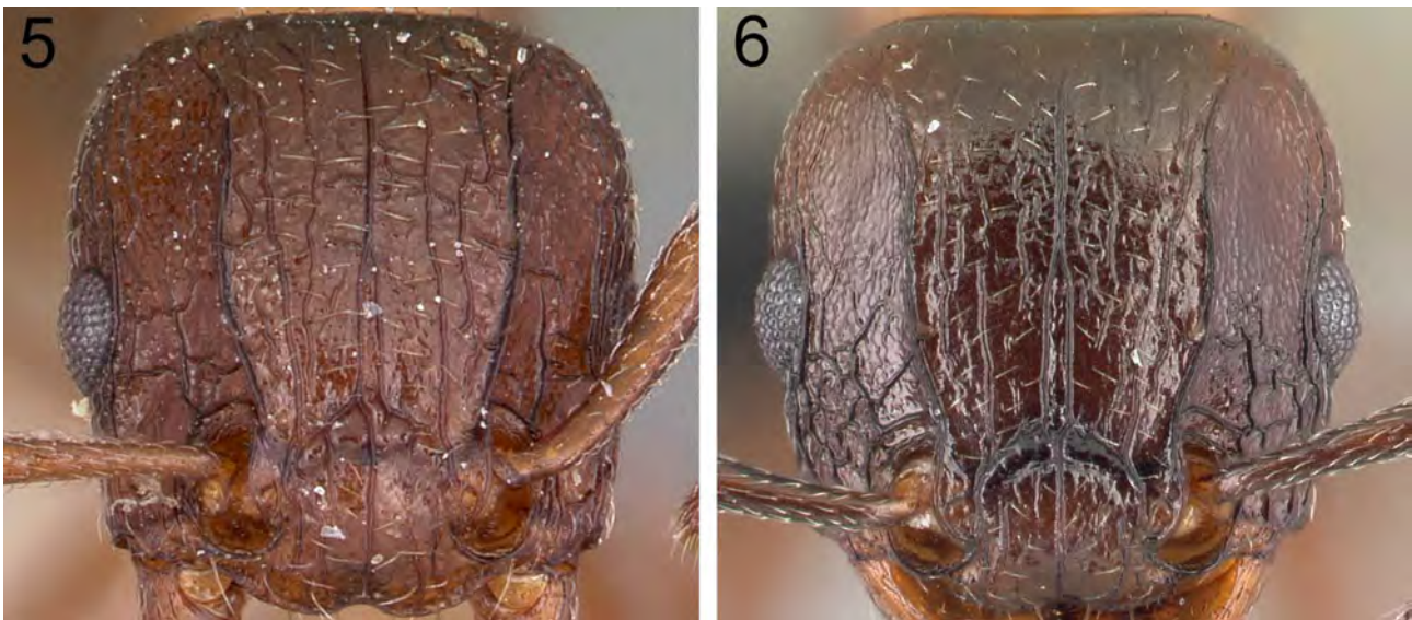
FIGURES 5 & 6. 5. Head of T. bessonii in full-face view, head shape distinctly longer than wide—CASENT0101298 (April Nobile 2006). 6. Head of T. wardi in full-face view, head shape approximately as long as wide—CASENT0475483 (Erin Prado 2010).
