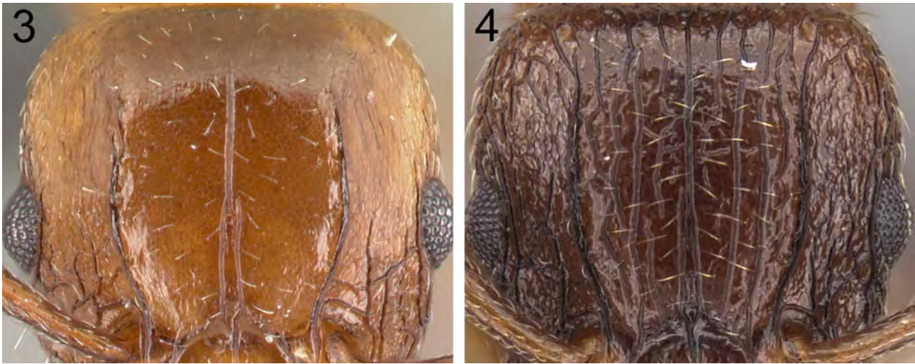
FIGURES 3 & 4. 3. Head of T. artemis in full-face view with one strongly developed median ruga between the frontal carinae—CASENT0481732 (Erin Prado 2010). 4. Head of T. bessonii in full-face view with strongly developed longitudinal median ruga and two to five more irregularly developed longitudinal rugae at each side—CASENT0247550 (Estella Ortega 2012).
