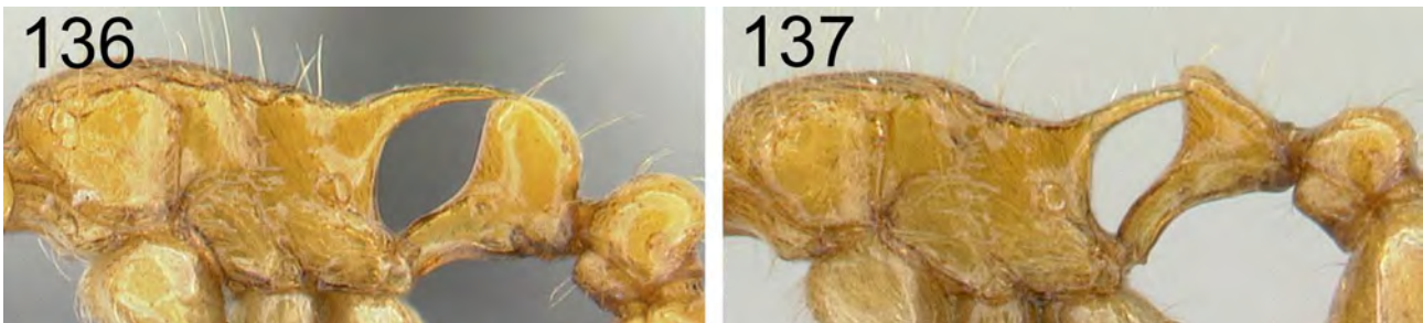
FIGURES 136 & 137. 136. Mesosoma and waist segments of T. shamshir in profile, propodeal spines strongly back-curved and petiolar node high nodiform to weakly cuneiform, not strongly anteroposteriorly compressed dorsally—CASENT0467696 (Erin Prado 2010). 137. Mesosoma and waist segments of T. norvigi in profile with triangular cuneiform and strongly anteroposteriorly compressed dorsally petiolar node—CASENT0489037 (Erin Prado 2010).
