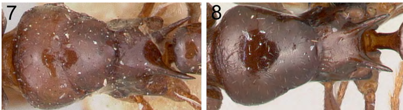
FIGURES 7 & 8. 7. Mesosoma of T. orientale in dorsal view showing the well-developed and conspicuous promesonotal suture—CASENT0101744 (April Nobile 2006). 8. Mesosoma of T. malagasy in dorsal view without a promesonotal suture—CASENT0449550 (Erin Prado 2010).
