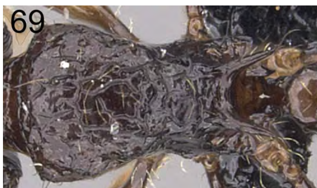
FIGURES 69 & 70. 69. Mesosomal dorsum of T. ambatovy in dorsal view showing the fine, irregularly arranged rugulae—CASENT0124721 (William Ericson 2011). 70. Mesosomal dorsum of T. steinheili with distinctly longitudinally arranged rugae—CASENT0101257 (April Nobile 2006).
