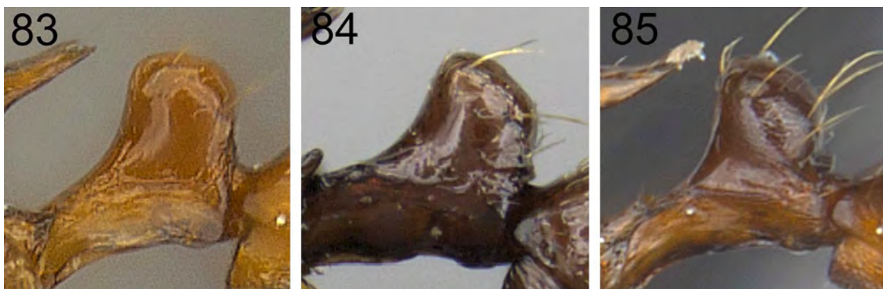
FIGURES 83–85. 83. High nodiform petiolar node of T. vohitra in profile, with anterodorsal and posterodorsal margins at approximately the same height and the dorsum not tapering backwards posteriorly—CASENT0218034 (Estella Ortega 2011). 84. High nodiform petiolar node of T. sargina in profile, with anterodorsal margin situated higher than posterodorsal margin and the dorsum tapering backwards posteriorly—CASENT0487390 (Estella Ortega 2011). 85. Squamiform petiolar node of T. steinheili in profile, with anterodorsal margin situated higher than posterodorsal margin and the dorsum tapering backwards posteriorly—CASENT0142632 (Estella Ortega 2011).
