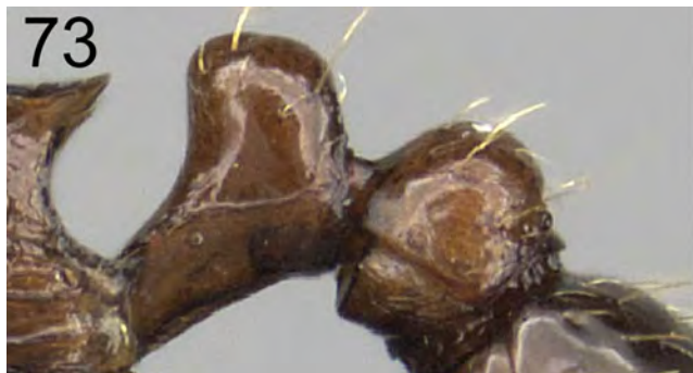
FIGURES 73 & 74. 73. Rounded high nodiform petiolar node of T. robitika in profile with anterodorsal and posterodorsal margins situated at approximately same height—CASENT0056338 (Estella Ortega 2011). 74. Petiolar node of T. orc in lateral view, shape moderately cuneiform with rounded margins, and anterodorsal margin situated higher than posterodorsal and dorsum tapering backwards posteriorly—CASENT0040573 (Estella Ortega 2011).
